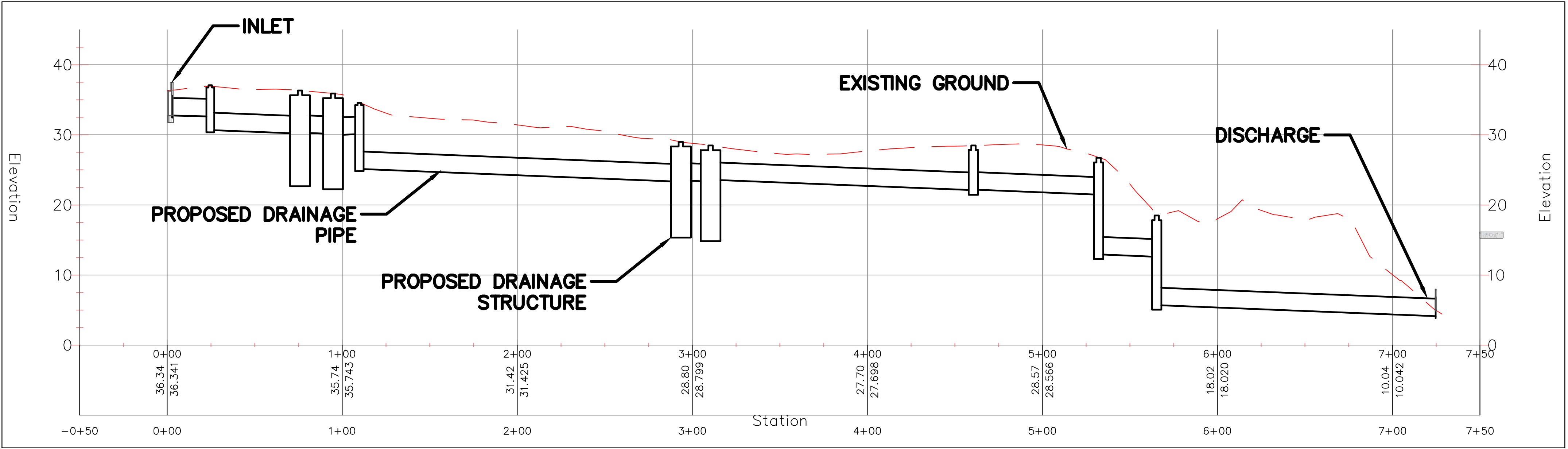
SCALE: 1"=40' HORIZONTAL 1"=10' VERTICAL
